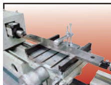
Long gauge block comparison calibration vertical & horizontal
