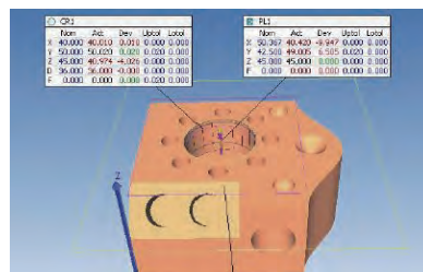
DMIS program input, output, editing and various report output
