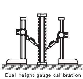
Dual height gauge calibration
