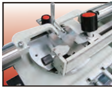
Setting inner thread with set gauge
