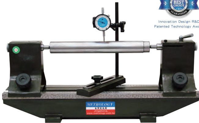
Measuring table and position device
