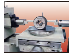
Inner thread gauge measurement with double yokes
