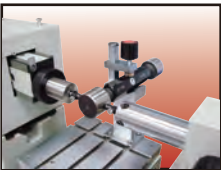
Plug gauge calibration with V-shaped carrier
