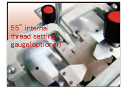
Setting zero for inner thread set gauge
