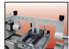
Medium size ring gauge calibration with inner double yokes
