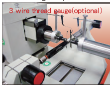
3 wire External thread gauge measurement with center carrier & V-type holder
