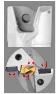
Patented pocket design
