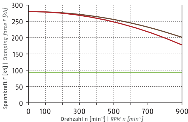
Clamping force-RPM-diagram
