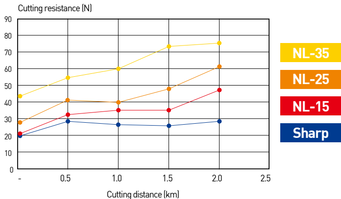
Comparison of cutting resistance
