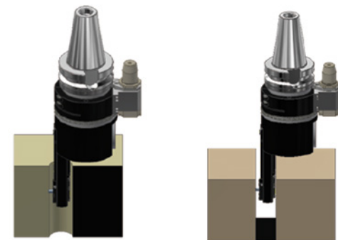
Min. \varnothing 40 Hole (except tool projection)
