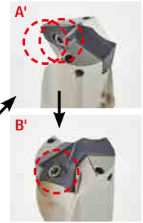
⑤ Clamp the screws completely in the order of A', B'.
