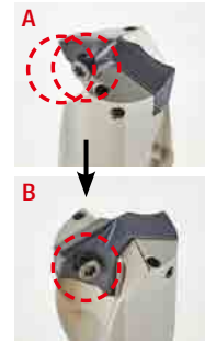
④ Clamp a screw partially just like in the case of A and B to prevent laterality.
