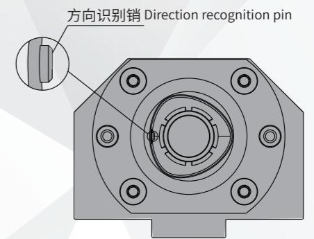
左刀座示例 Example of left hand holder
