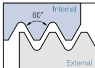
Partial profile 60°
